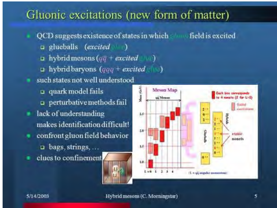
Figure 3.1: Spectrum of mesons (as anticipated by lattice calculations as well as QCD-inspired modeling) in the mass range of 1.5 to 2.7 GeV. Those nonets with J^{PC} quantum numbers that cannot simply be qq systems (often called "exotic") are labeled in red on the right.
