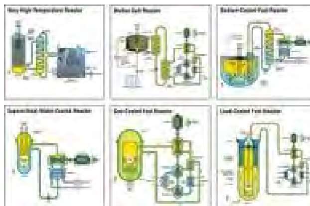
Figure 8.5: The six technologies investigated in GIF. From [6]
