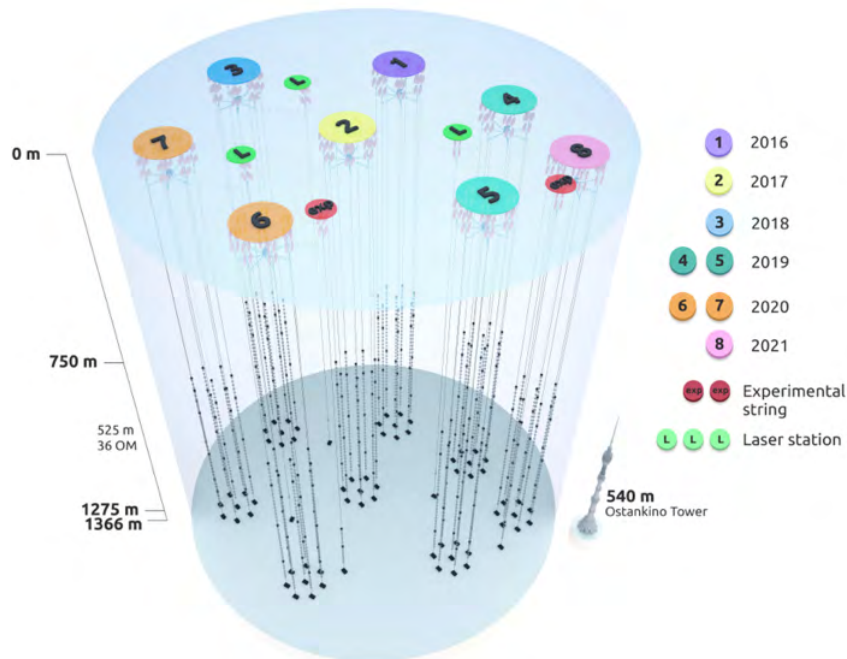
Figure 13.79: Baikal-GVD detector.
