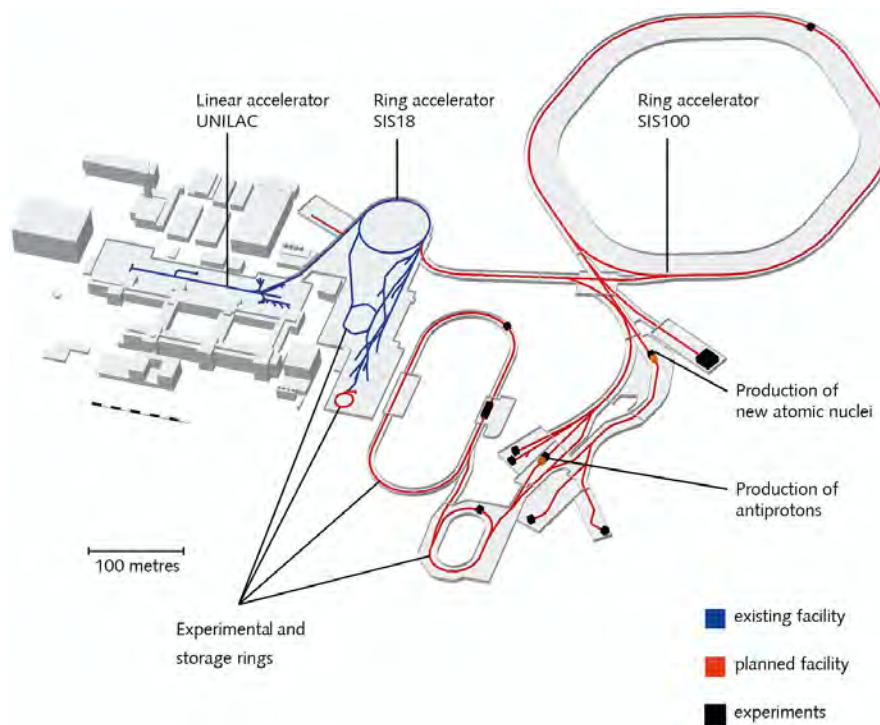
Figure 13.22: Major facilities of GSI and FAIR. (c) GSI
