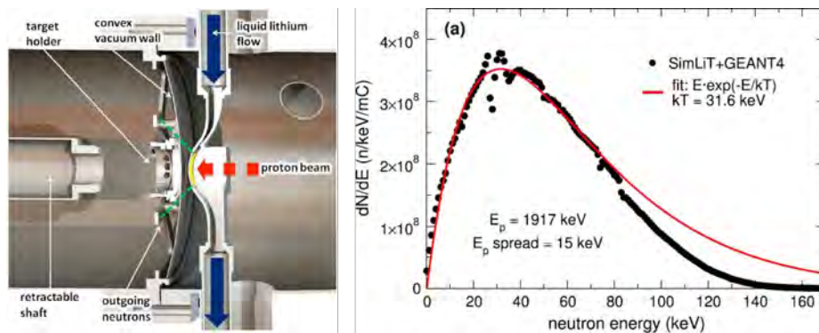
Figure 13.39: (Left) Cross section of LiLiT near the nozzle. The sample to be irradiated by the neutrons is placed at 6 mm from the target [2]. (Right) Typical neutron spectrum from LiLiT [3].
