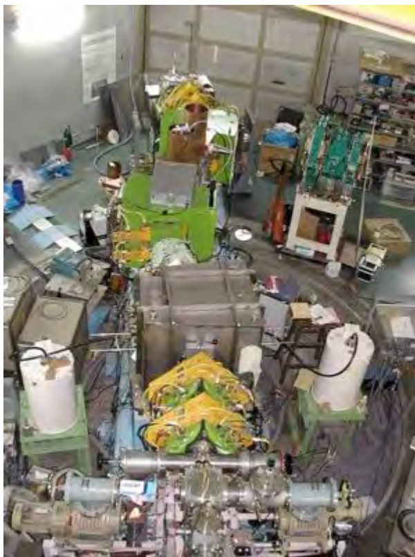
Figure 11.18: A recoil mass separator consisting of QQEMDDQQ (upper part) and a windowless gas target (lower part) for astro-nuclear experiments.
