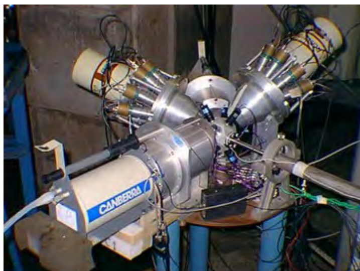
Figure 15.5: The SACI-PERERE gamma-ray spectrometer.
