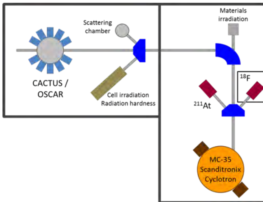
Figure 13.57: Experimental areas at OCL.
