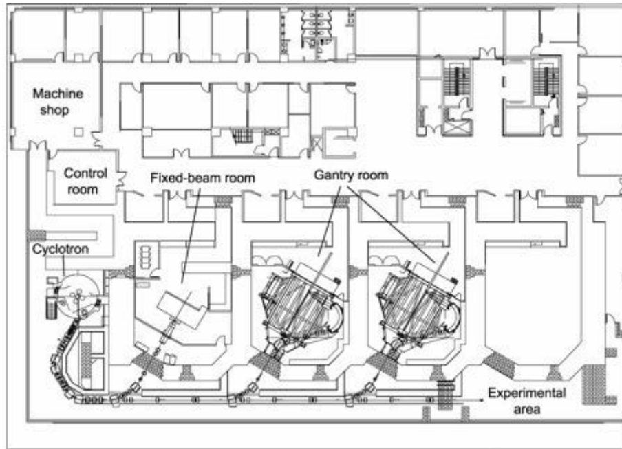
Figure 11.28: Experimental areas at the Center for Proton Therapy.
