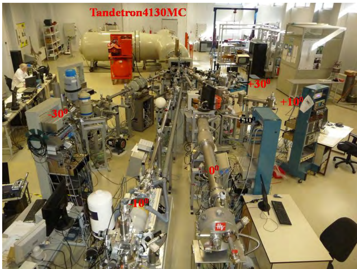
Figure 13.5: Photo of the Tandetron 4130MC with associated beam lines.
