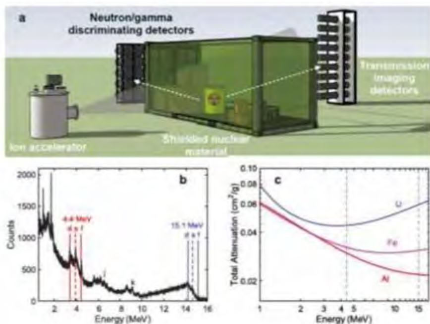
Figure 6.3: Detecting illicit weapon trafficking. (a) Low-energy nuclear reaction imaging relies upon the source of monochromatic photons via a nuclear reaction between an ion accelerated to MeV-scale energy and a target. Gamma rays at discrete energies are produced from nuclear excited states of the product nucleus, with some reactions also producing neutrons. The collimated, penetrating radiation from the nuclear reaction source is used to perform transmission radiography of a shielded object, while neutron/gamma discriminating detectors detect the signature of nuclear fission. (b) Photon spectrum from the ^{11}\text{B}(d, n\gamma)^{12}\text{C} reaction measured with a LaBr scintillation detector. (c) Energy-dependent attenuation for several elements. The 4.438 MeV and 15.1 MeV gamma energies from the ^{11}\text{B}(d, n\gamma)^{12}\text{C} reaction are shown as dashed lines (Rose et al., Sci. Rep. 6:24388, 2016).
