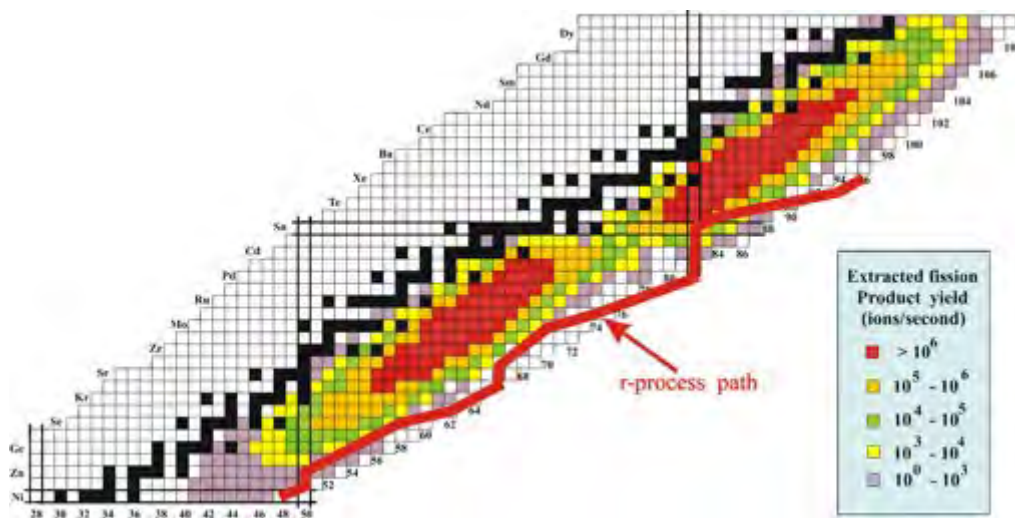
Figure 14.12: Fission yield distribution for a thin 1 Ci ^{252}\text{Cf} source in ions/s. Stopped beam total efficiency to target is approximately 40%. For accelerated beams with ATLAS, total efficiency to target, including charge breeding efficiency, is approximately 5%.
