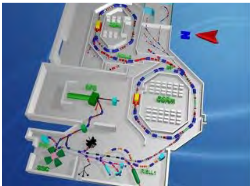
Figure 11.2: Schematics of the facilities in Lanzhou.
