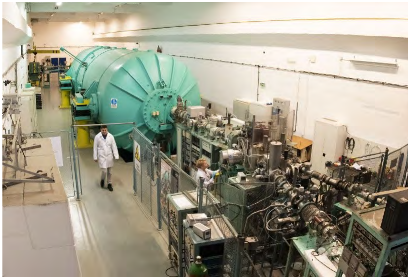
Figure 13.66: The 9-MV Tandem.
