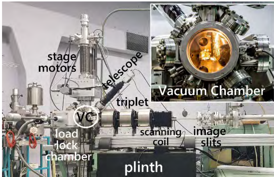
Figure 13.34: (Left) The nuclear microprobe (see also [1]). (Right) : The external ion beam setup.
