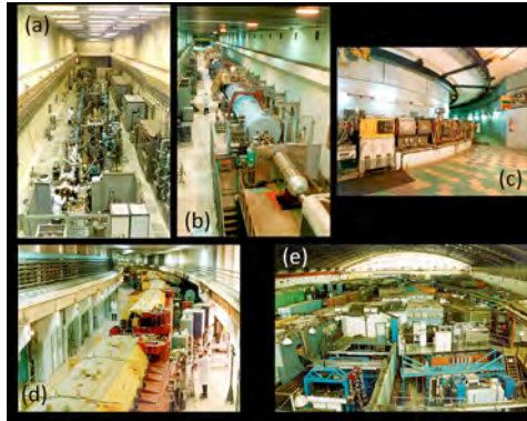
Figure 13.76: IHEP facilities: (a) Proton Linac RFQ DTL URAL-30; (b) Alvarez DTL I-100; (c) Booster RCS U-1.5; (d) U-70 synchrotron; (e) Main experimental hall with beam-lines and detectors.
