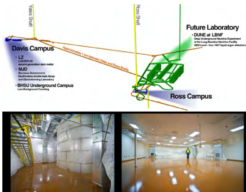
Figure 14.26: The SURF 4850 level highlighting existing campuses (blue shading), as well as LBNF/DUNE caverns currently under construction (green shading). Pictures of space at the Davis Campus are also shown.
