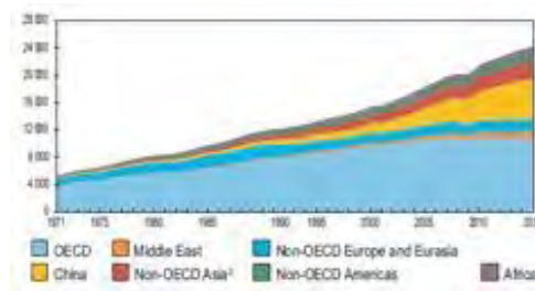
Figure 8.2: World electricity generation from 1971 to 2015 by region (TWh). From [3].
