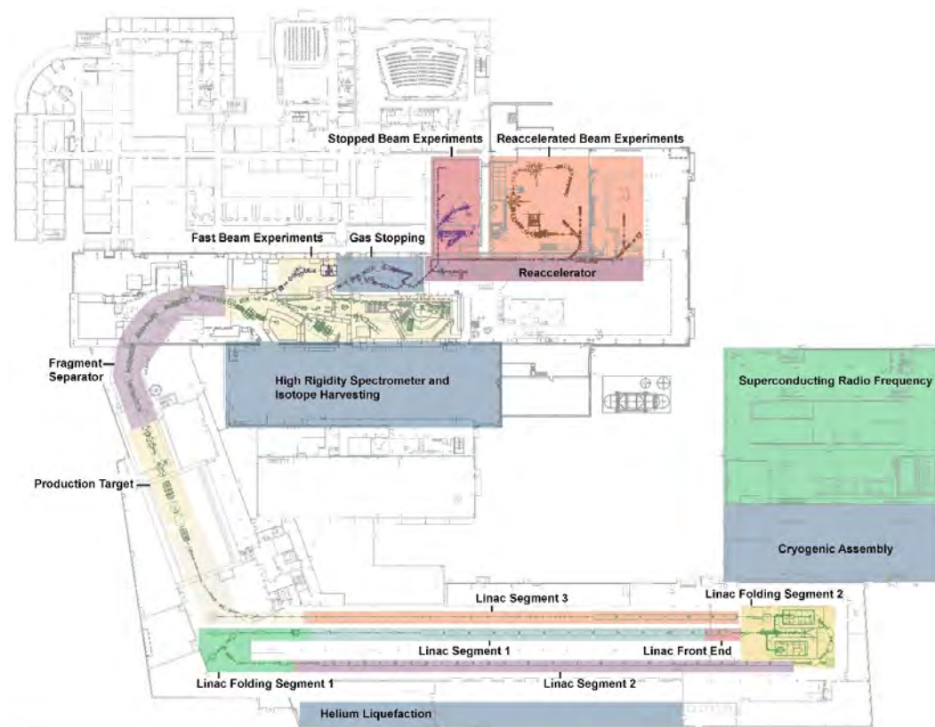
Figure 14.21: FRIB facility layout.
