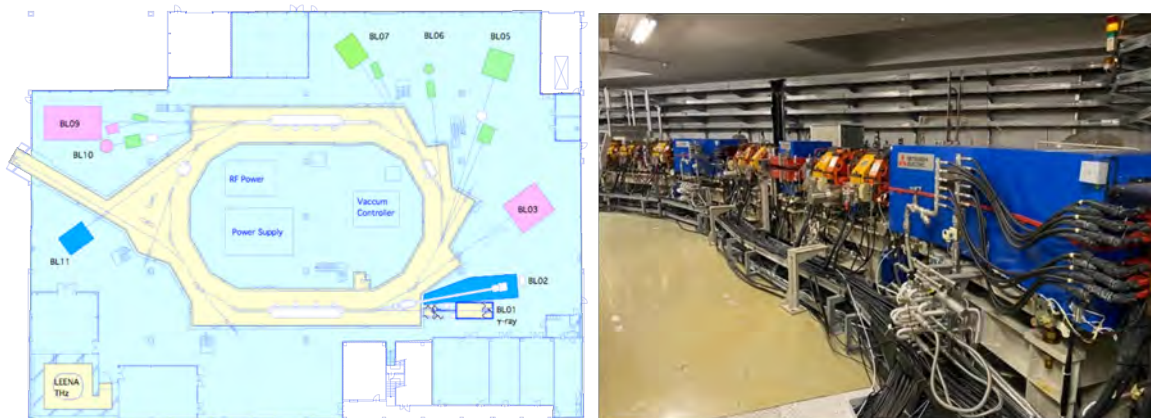
Figure 11.13: Layout of NewSUBARU synchrotron light facility (left). Gamma-ray beam line is BL01. An electron beam is injected from 1 GeV linac. The electron storage ring (right) is operated with a top-up current of 350 mA. Natural emittance of the electron beam is 37 nm-rad. The circumference of the storage ring is 118.73 m, the RF frequency and number of electron buckets are 500 MHz and 198, respectively.
