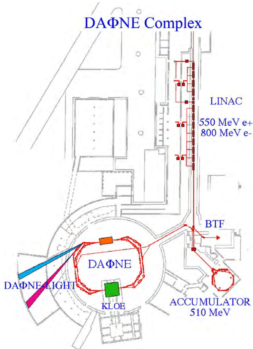
Figure 13.52: Picture of the DAΦNE complex.
