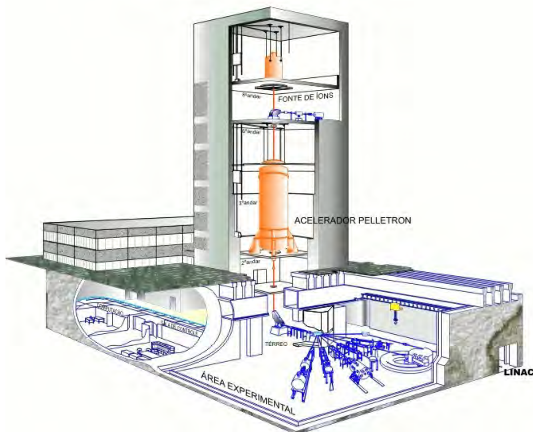
Figure 15.3: The 8 UD Pelletron Tandem accelerator.
