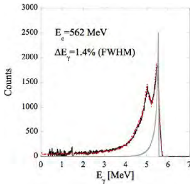
Figure 11.15: This shows a spectra of LCS \gamma -ray with the Nd:YVO4 laser (wavelength of 1064 nm) scattered with electron beam of 562 MeV measured by a LaBr3 (Ce) detector [Ref]. The LCS \gamma -ray was collimated with a lead block of 10 cm thick with 2mm diameter hole located at 16.7 m from the collision point. Quasi-monochromatic \gamma -ray beam with energy spread of 1.4% is obtained. A experimental response function (solid line) of the LaBr3 (Ce) detector along with the simulated response function (dotted line) and energy distribution of the LCS \gamma -ray beam (grey line). [Ref] Utsunomiya et al. Phys. Rev. C 92, 064323 (2015).
