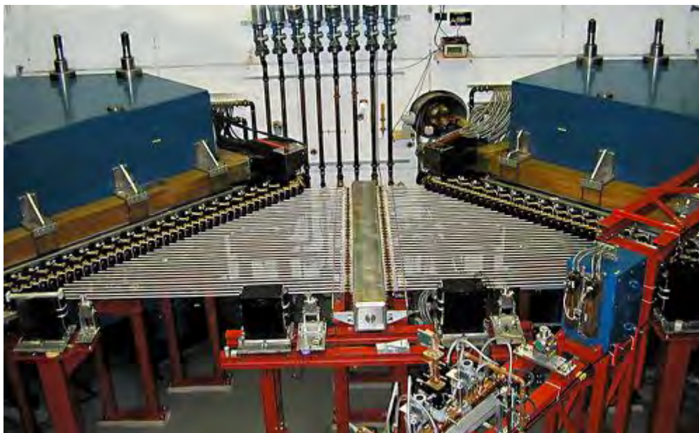
Figure 13.25: Picture of the latest microtron stage MAMI-C. A maximum electron beam energy of 1.604 GeV can be achieved.
