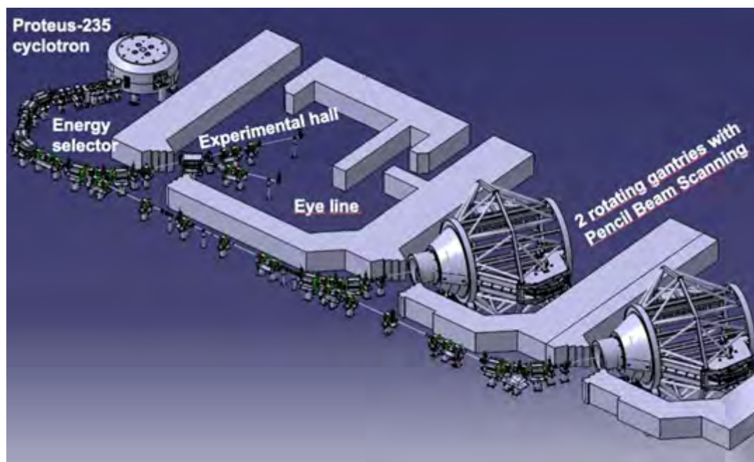
Figure 13.58: Experimental areas at IFJ PAN Krakow.
