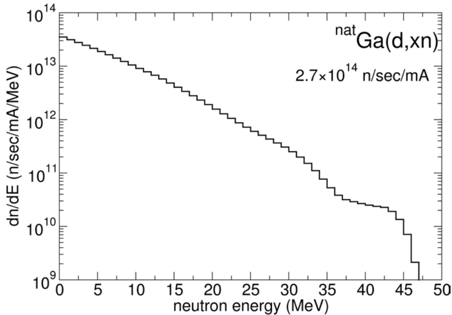
Figure 13.45: Simulated neutron energy spectrum from ^{nat}\text{Ga} , the main component (more than 80% of the atoms) of the liquid GaIn target, when irradiated by 40 MeV deuterons. The energy-integrated neutron rate per mA of deuterons is given within the plot. We assume only an S-wave contribution, which is considered the dominant component.
