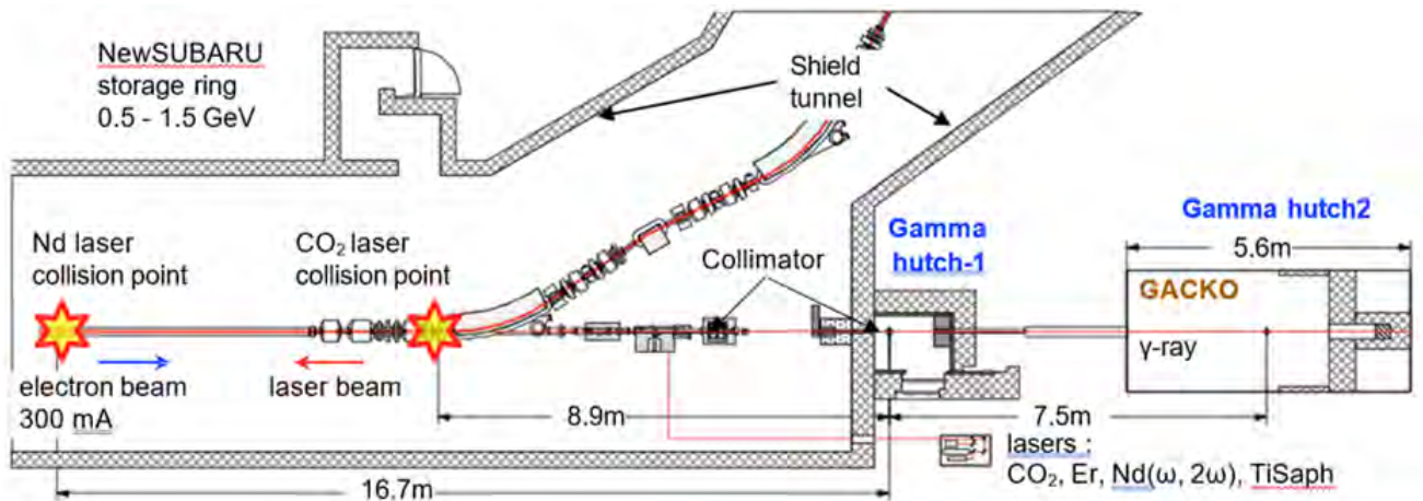
Figure 11.14: A 1/6 of NewSUBARU electron storage ring is shown. Laser injection is made from the outside of the shield tunnel of the storage ring. Electron beam and the laser beam collide at two collision points depend on the laser wavelength. LCS-gamma-ray beam propagate to the gamma-ray hutches pass through the vacuum window. Two gamma-ray hutches are arranged in series.
