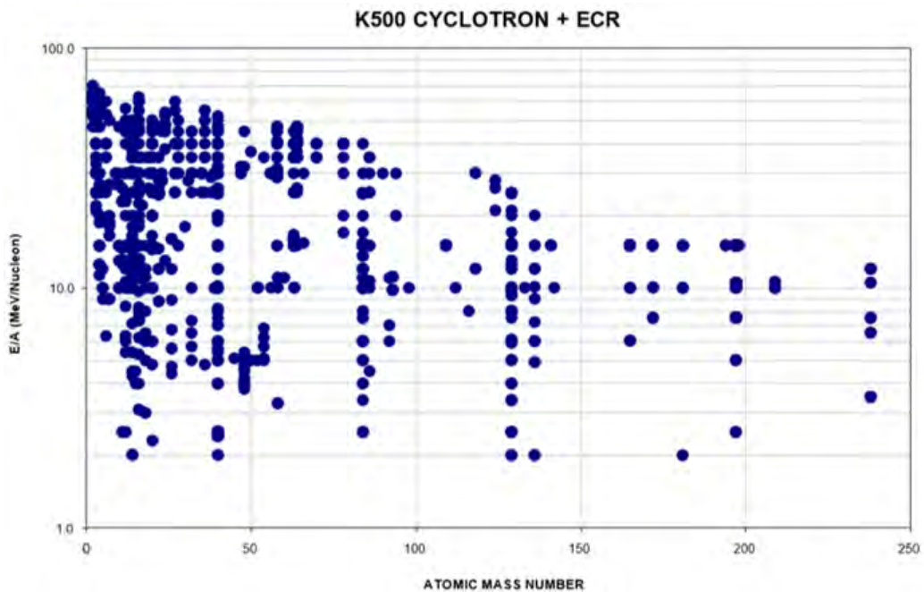
Figure 14.17: Available beams from the K500.
