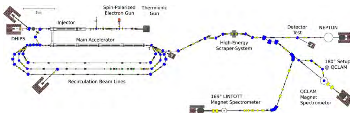
Figure 13.20: Floorplan of the S-DALINAC with its experimental setups.
