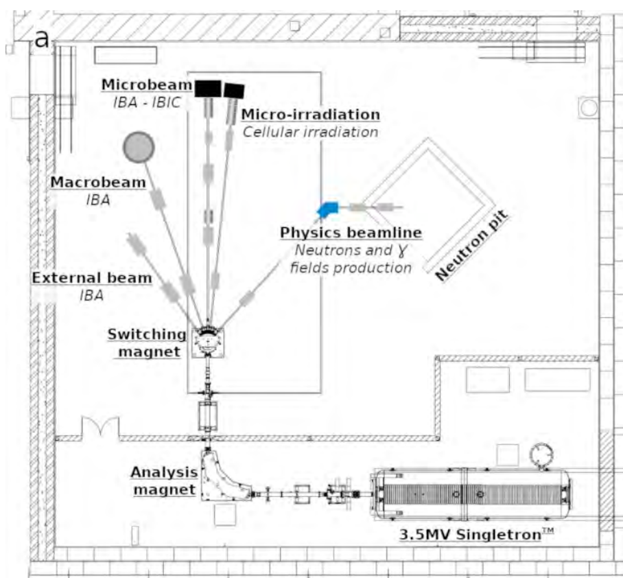
Figure 13.12: Overview of the AIFIRA facility.
