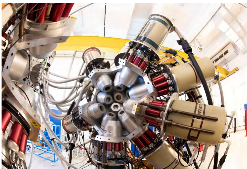
Figure 13.67: The ROSPHERE \gamma array.
