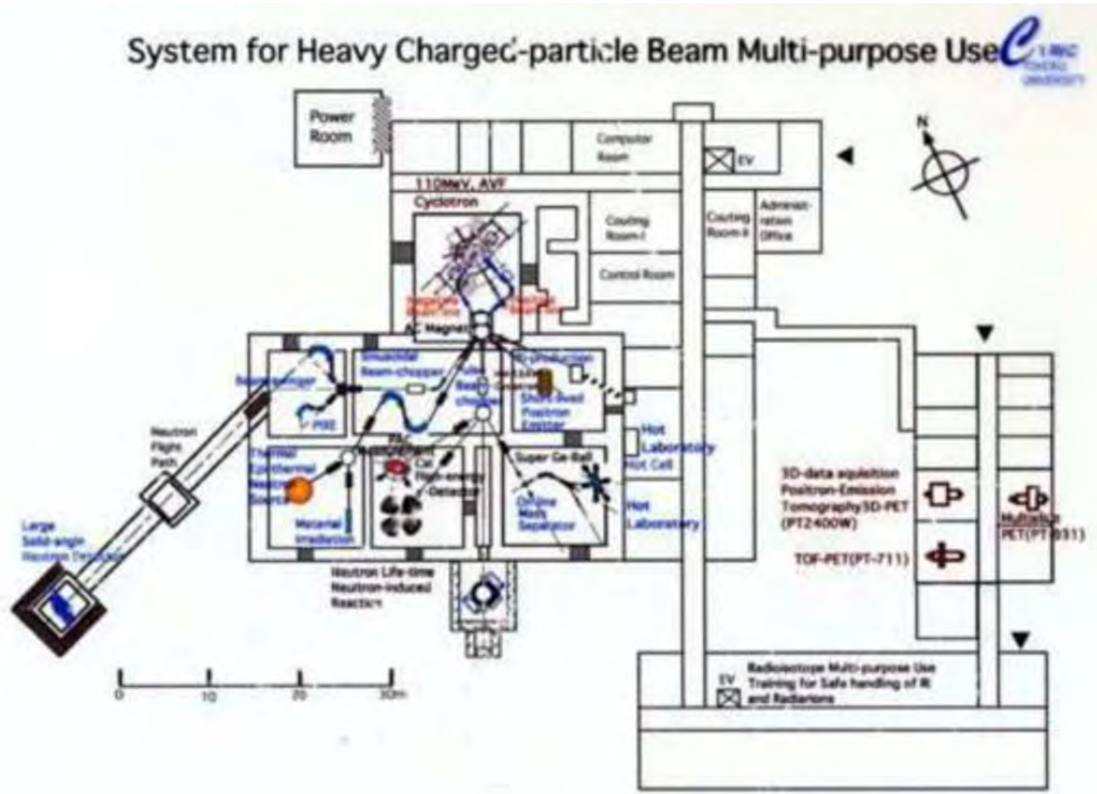
Figure 11.23: Experimental areas at CYRIC.
