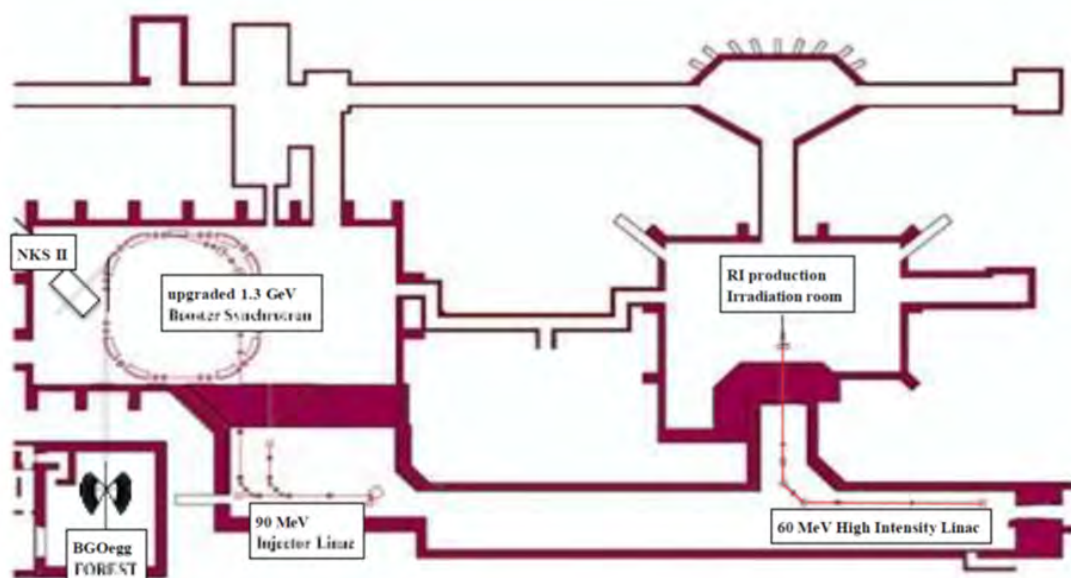
Figure 11.20: ELPH Accelerator Facilities.
