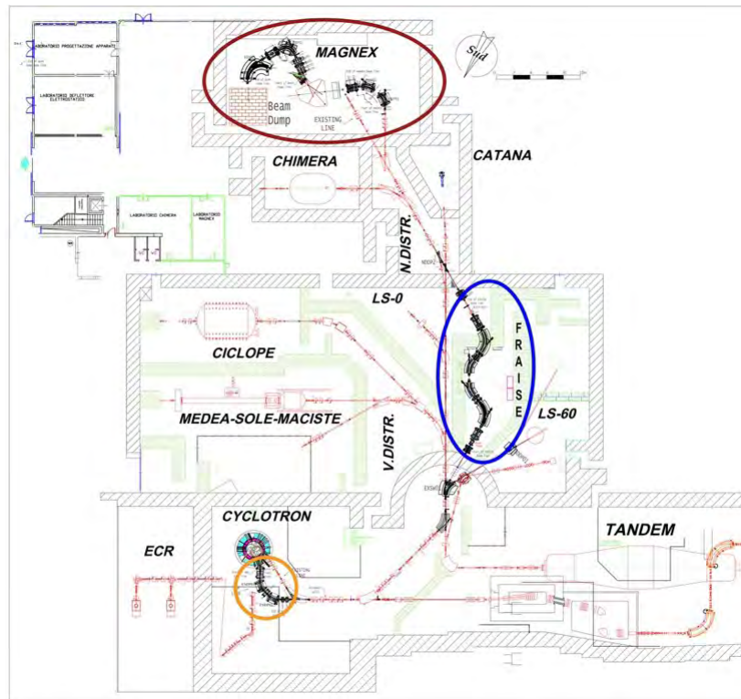
Figure 13.50: Schematic layout of LNS beamlines.
