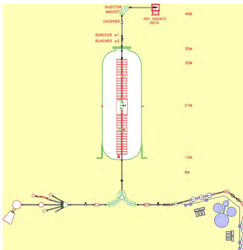
Figure 11.8: Schematic layout of 14MV Pelletron accelerator and LINAC
