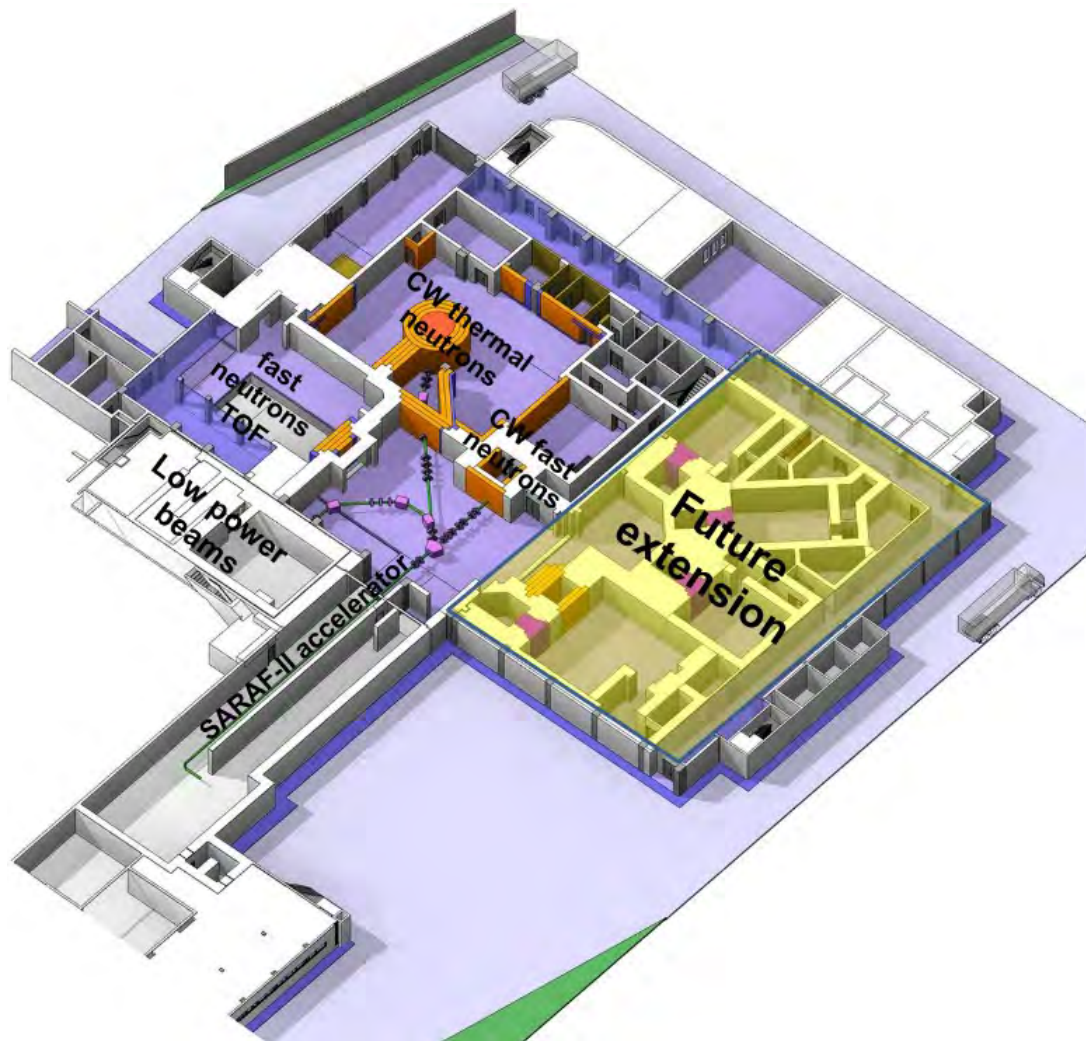
Figure 13.43: Layout of the SARAF-II target hall. The four irradiation areas are described in the text. The yellow-highlighted part is a future extension that is not built yet.
