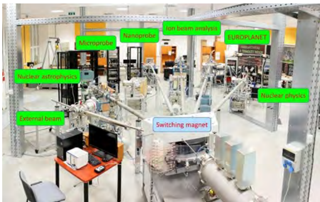
Figure 13.37: Beamlines at ATOMKI.
