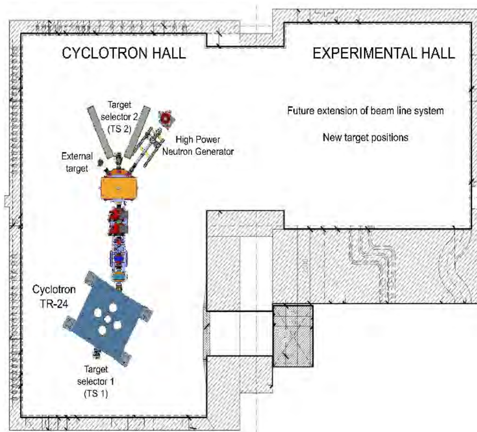
Figure 13.2: Layout of the TR-24 Cyclotron.
