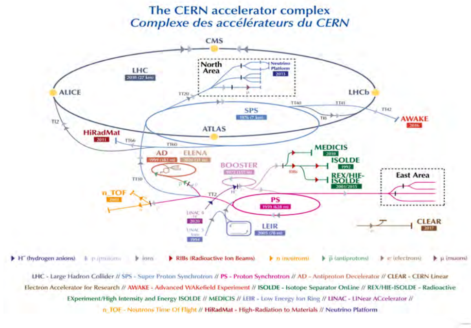
Figure 13.93: Accelerator complex at CERN (Image: CERN).
