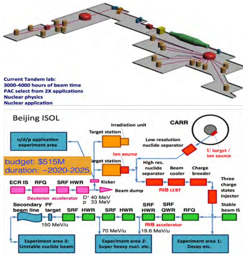
Figure 11.1: Schematic drawing of the current and future facilities in Beijing.
