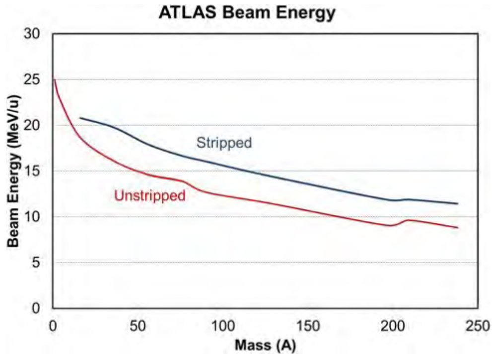
Figure 14.11: Maximum beam energy from ATLAS as a function of ion mass for two stripping assumptions. In general stripped beams will have approximately 20% of the intensity of unstripped beams.
