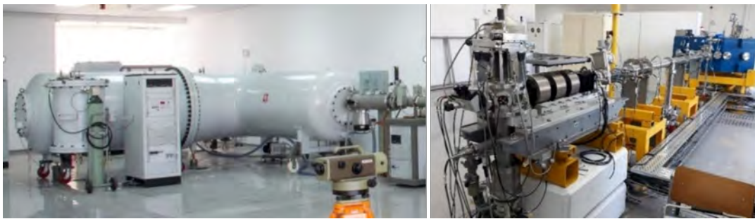
Figure 10.1: The 3-MV Tandetron accelerator (left) and its micro-probe setup (right).
