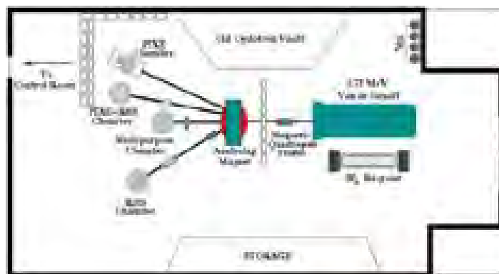
Figure 15.8: Layout of the Van de Graaff facility.
