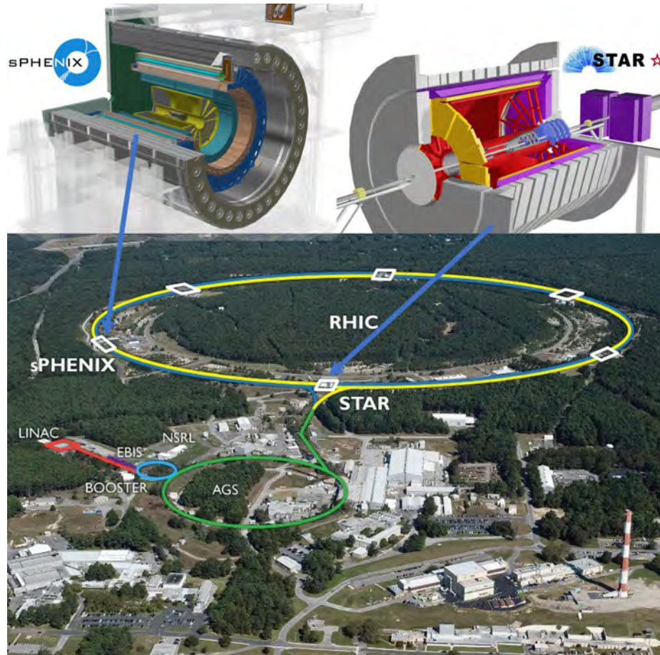
Figure 14.23: Layout of RHIC and illustration of its two principal detectors, STAR and sPHENIX.
