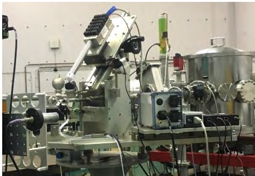
Figure 13.35: The RBS/Channeling chamber and the sample manipulator translations and rotations.
