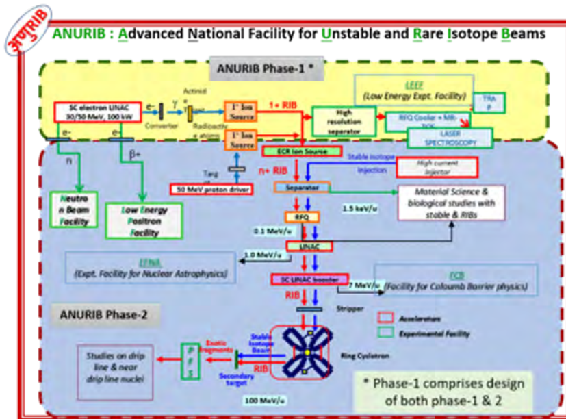
Figure 11.6: RIB facilities at VECC.
