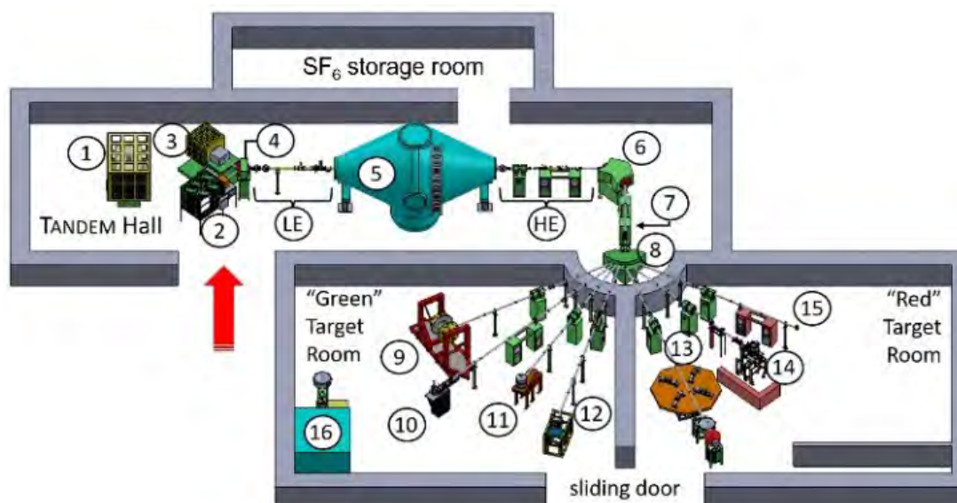
Figure 13.29: Schematic layout of the Tandem-hall and the two target rooms of the laboratory. The main accelerator components and setups are described in Fig. 13.28.
