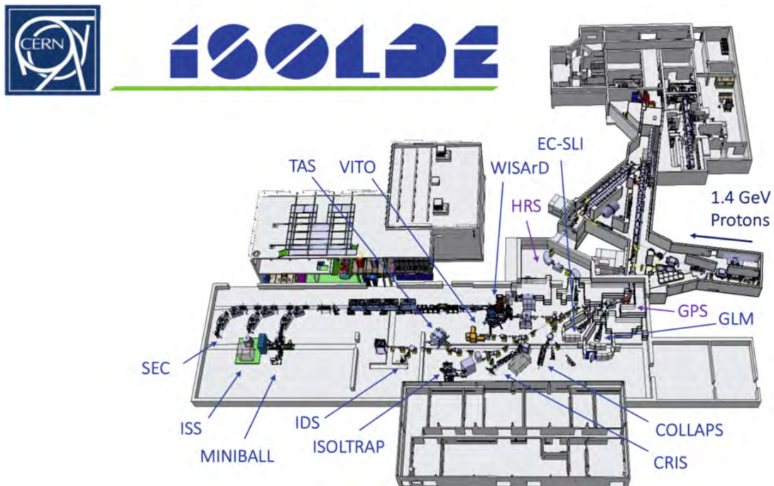
Figure 13.92: The ISOLDE facility showing the two mass separators and major instrumentation (see table below).
