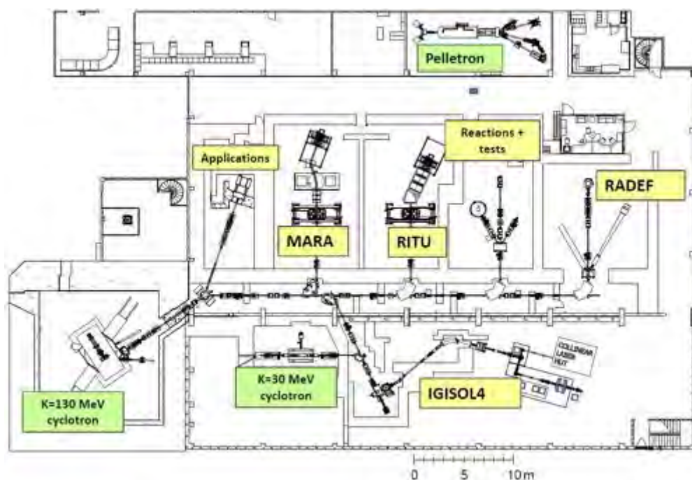
Figure 13.8: Layout of the upgraded JYFL Accelerator Laboratory.
