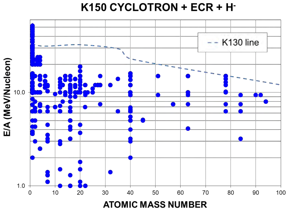
Figure 14.18: Available beams from the K150.
