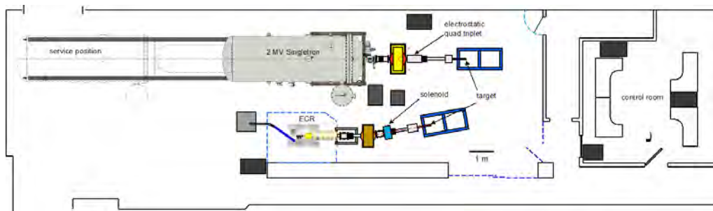
Figure 14.32: Layout of LENA
