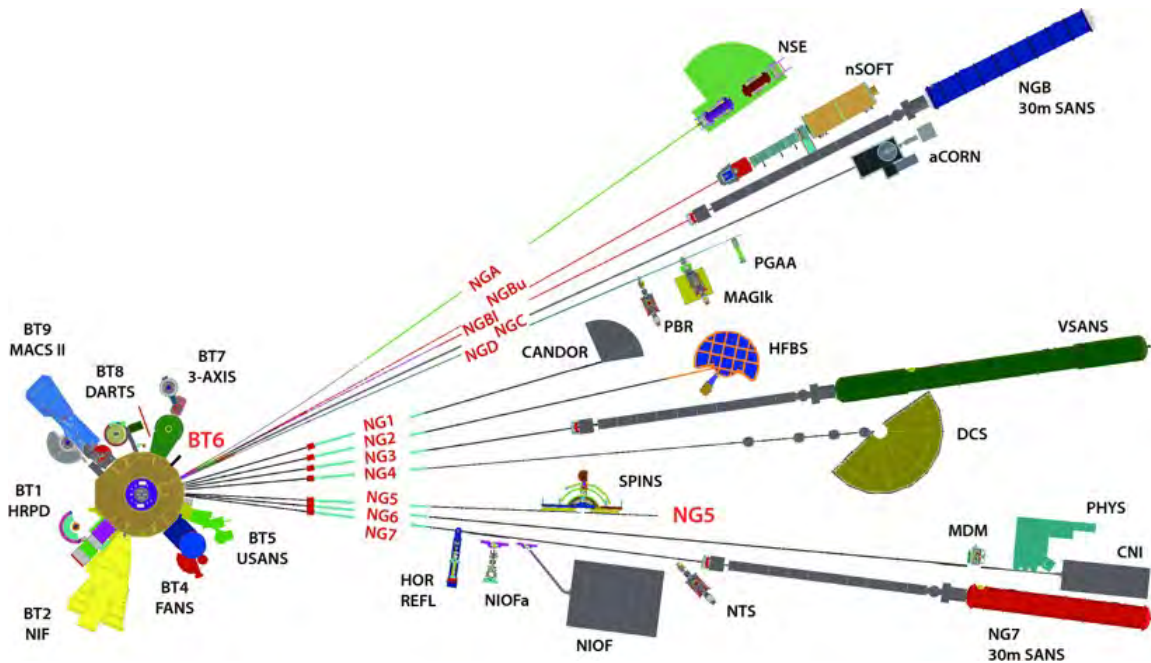
Figure 14.22: Beamlines at NIST.
