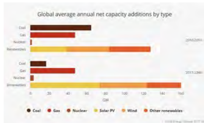
Figure 8.3: Global average annual net capacity additions by type of fuel during the 2010-2016 period and foreseen by IEA between 2017 and 2040. From [2].
