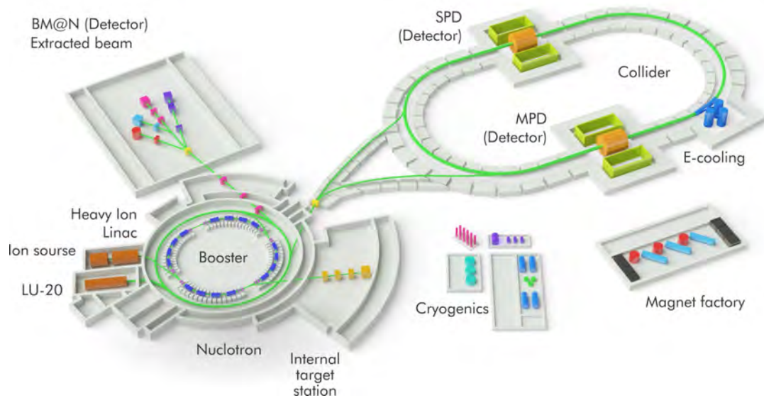
Figure 13.84: Layout of the NICA complex.
