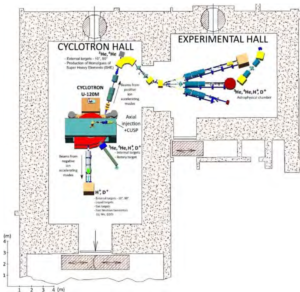
Figure 13.1: Layout of the U-120M Isochronous Cyclotron.
