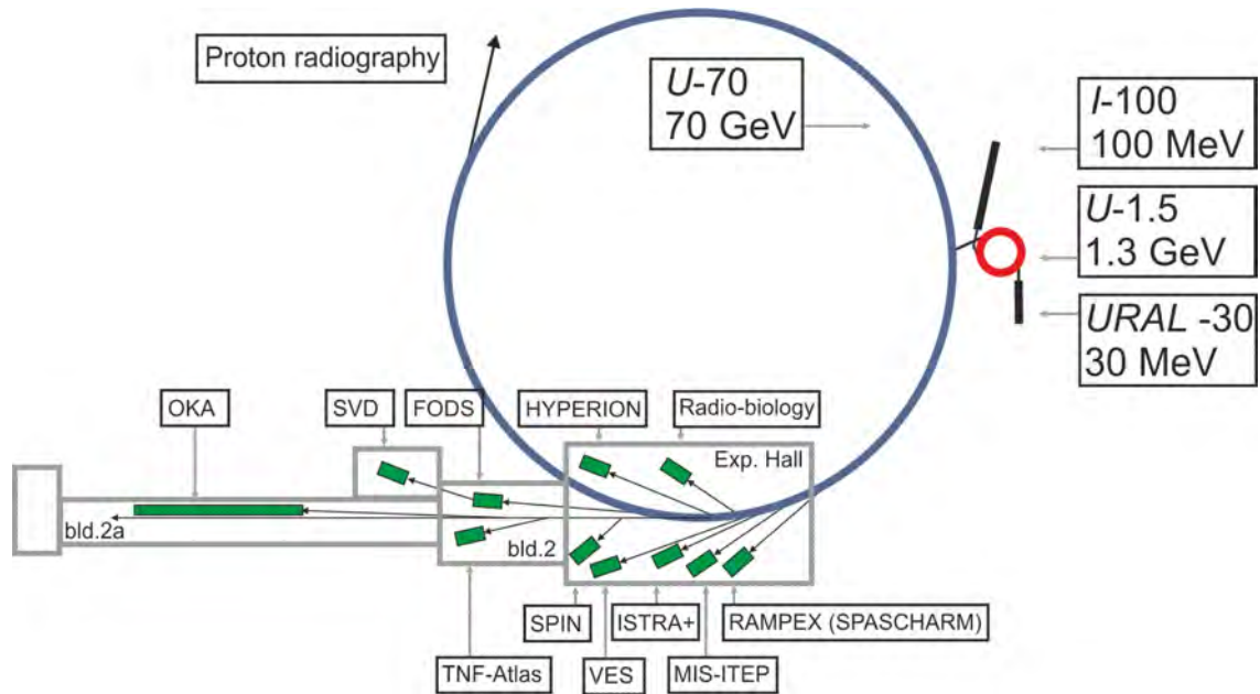
Figure 13.72: Experimental areas at IHEP.
