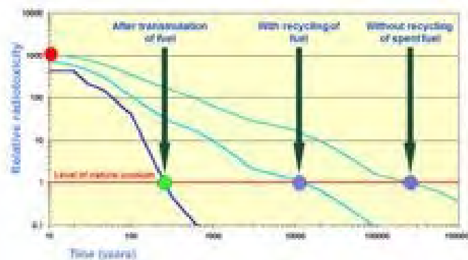
Figure 8.6: Relative radiotoxicity on nuclear waste compared to natural uranium ore as a function of time after unloading from the reactor, for spent fuel without recycling, with Pu recycling and after transmutation of minor actinides. From [8, 9].
