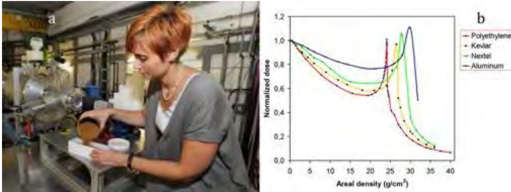
Figure 6.2: Space radiation shielding tests. Accelerator tests of the shielding effectiveness of different space relevant materials. (a) Mars regolith is prepared at the GSI accelerator in Germany. (b) Measured Bragg curves.
