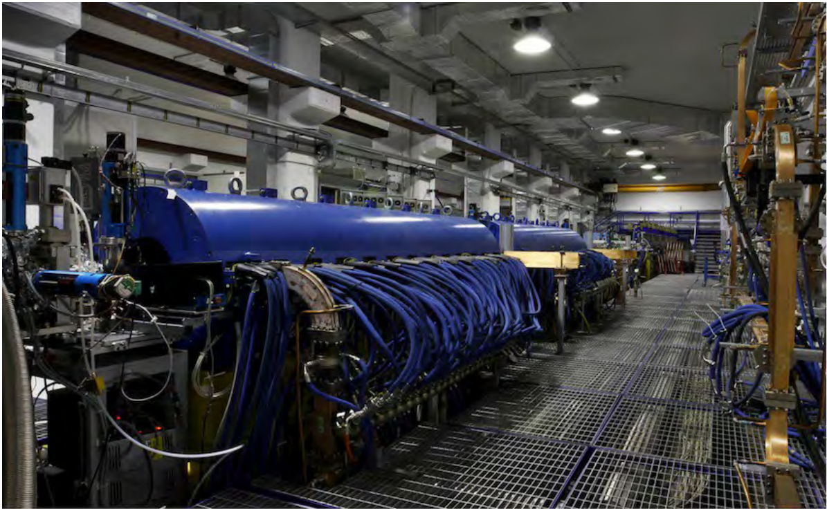
Figure 13.53: Beamline at LNF.
