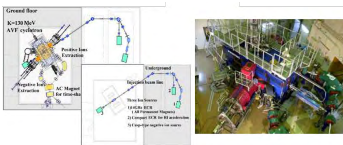
Figure 11.22: Overview of the facilities at CYRIC.
