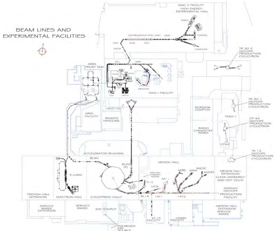
Figure 14.3: Beam lines and experimental facilities at TRIUMF.
