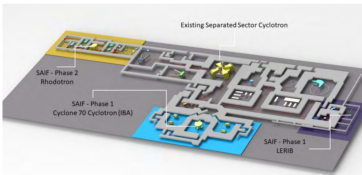
Figure 10.3: Layout of the facilities showing the current SSC and experimental vaults, the locations for the new C70 MeV cyclotron (light blue area) with the four irradiation target systems for radioisotope production, the LERIB0 facility (light purple) using the high-intensity 66 MeV proton beam from the SSC, and phase 2 of SAIF with the Rhodotron (light orange) for rare isotopes production (at low energy and high energy using the SSC accelerator) and for the production of high intensity neutron and photons source.
