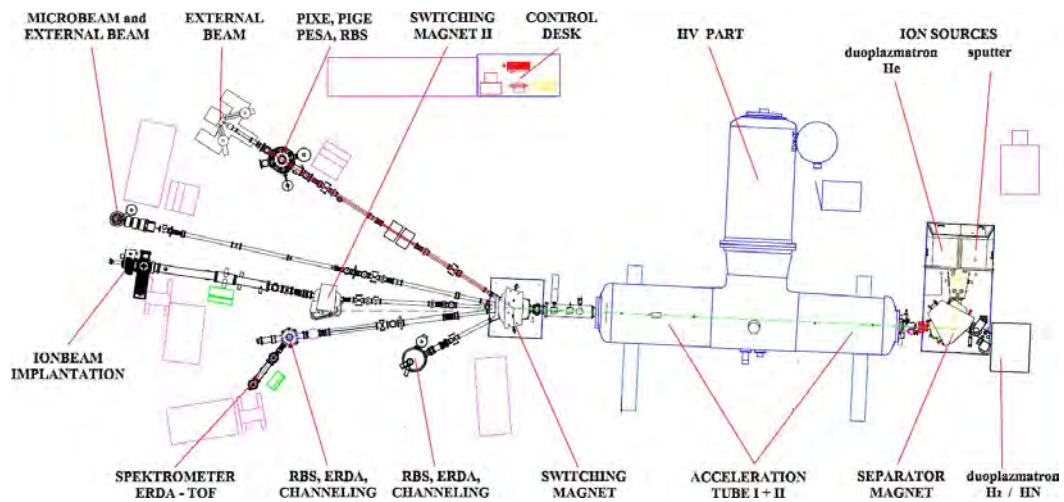
Figure 13.4: Layout of the Tandetron 4130MC.
