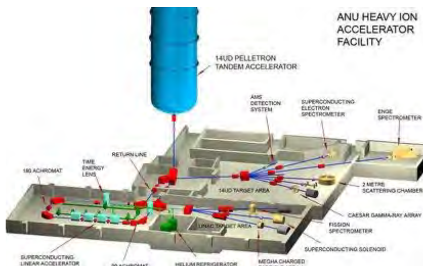
Figure 12.2: ANU Heavy Ion Accelerator Facility: General Layout.
