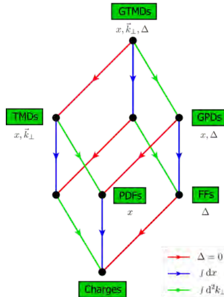
Figure 3.3: Complete set of parton distributions and their interrelations. \Delta is the Fourier conjugate variable to position.
