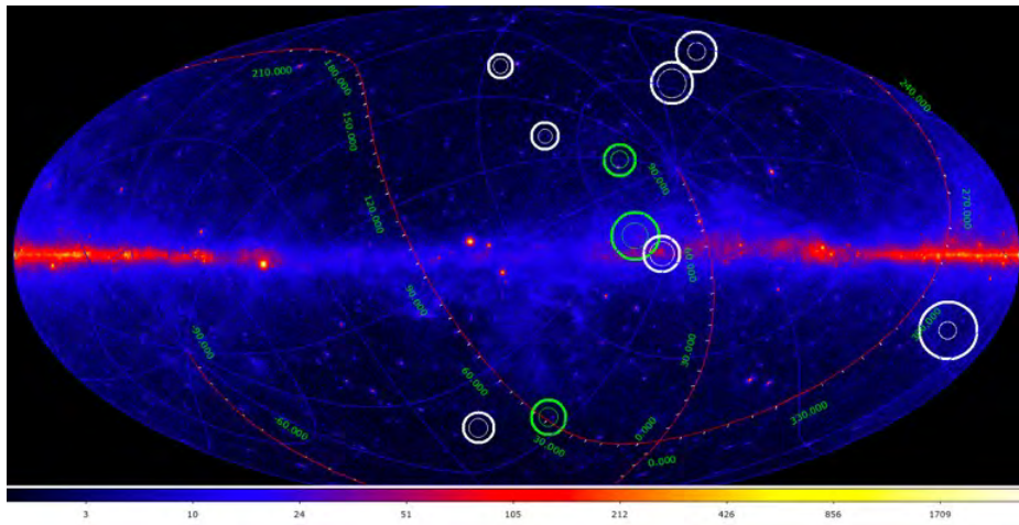
Figure 13.81: Positions of gamma sources and the first ten Baikal- GVD candidates for the astrophysical neutrino events are shown on the celestial sphere. The coordinate grid in the figure corresponds to the equatorial coordinate system. The inner and outer circles around the events correspond to a 50% and 90% probability of registration.
