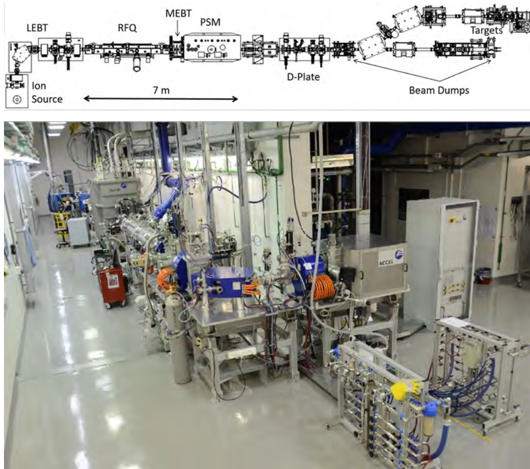
Figure 13.38: Top: Layout of SARAF-I [1]. Bottom: Photo of SARAF-I.
