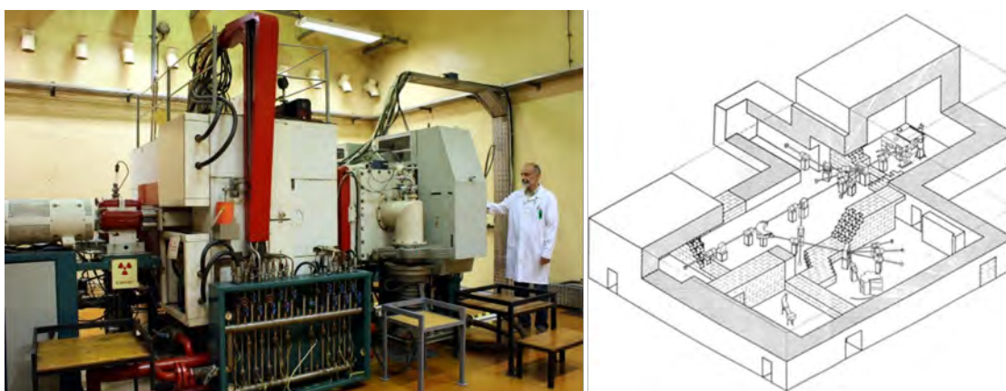
Figure 13.36: Experimental areas at ATOMKI.
