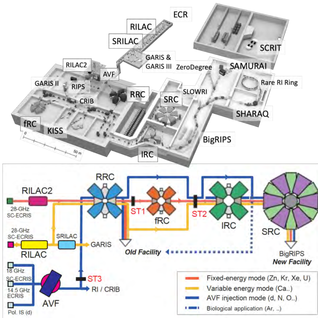
Figure 11.17: Layout of the present facility and RI Beam Facility and acceleration scheme.
