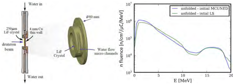
Figure 13.40: (Left) A CAD drawing of LiFTiT. Left: transverse cross section. Right: 3D depiction of the LiF crystal and the copper back [1]. (Right) - Unfolded spectra of LiFTiT by using different initial guess spectra. Spectra are normalized to reflect the neutron spectrum at 6 cm distance from the target [1].
