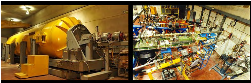
Figure 14.4: View of the Tandem Van de Graaff accelerator tank and experimental setups.
