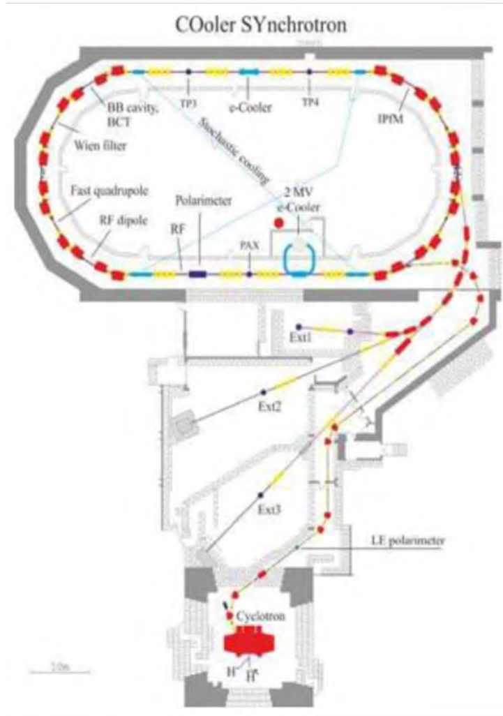
Figure 13.18: Experimental areas at COSY.
