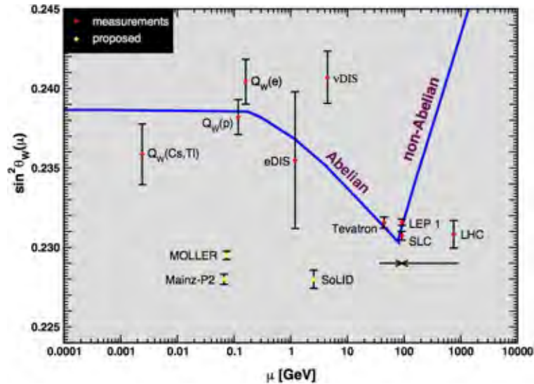
Figure 5.1: Calculated running of the weak mixing angle in the SM, as defined in the modified minimal subtraction scheme. The theoretical uncertainty is below the thickness of the blue curve. Red points with error bars show existing data and yellow points (with arbitrarily chosen ordinates) refer to future experiments. Q_W(\text{Cs, Tl}) derives from atomic parity violation, Q_W(p) from Qweak, and Q_W(e) from SLAC-E158, while vDIS and eDIS denote deep inelastic neutrino (NuTeV at Fermilab) and electron scattering, respectively.
