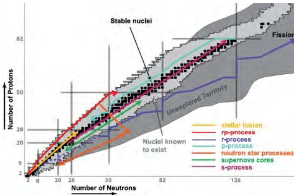
Figure 2.3: Nucleosynthesis processes across the nuclear chart. For most, the reactions and decay properties of rare isotopes are critical to understand the abundance patterns left behind [Figure from F. Timmes].
