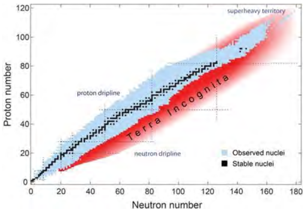
Figure 2.1: The nuclear territory – Black: stable nuclei; blue: nuclei known to exist; red: Nuclei that will still be discovered. The chart of nuclei is bounded by the nucleon driplines where no additional nucleons can be bound. Superheavy nuclei reside at the limit of charge and mass. A vast, unknown, and still uncertain part of the nuclear chart, the Terra Incognita, remains unexplored.
