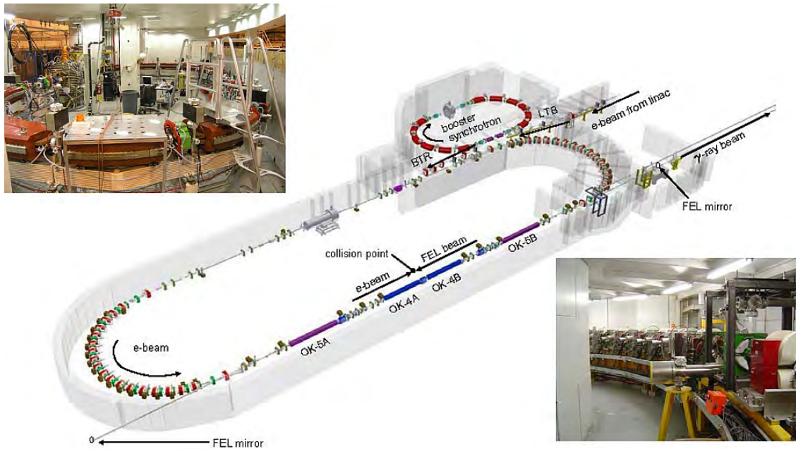
Figure 14.31: Layout of the HIGS accelerator systems with photographs of the booster (upper left) and a section of the electron storage ring (lower right).
