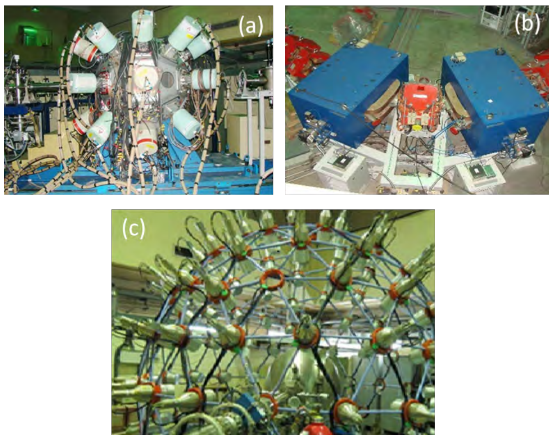
Figure 11.4: Facilities at IUAC: (a) Indian National Gamma Array; (b) Hybrid Recoil Mass Analyser; (c) National Array of Neutron Detectors.
