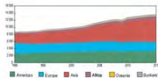
Figure 8.1: World total primary energy supply by geographical region. From [3].
