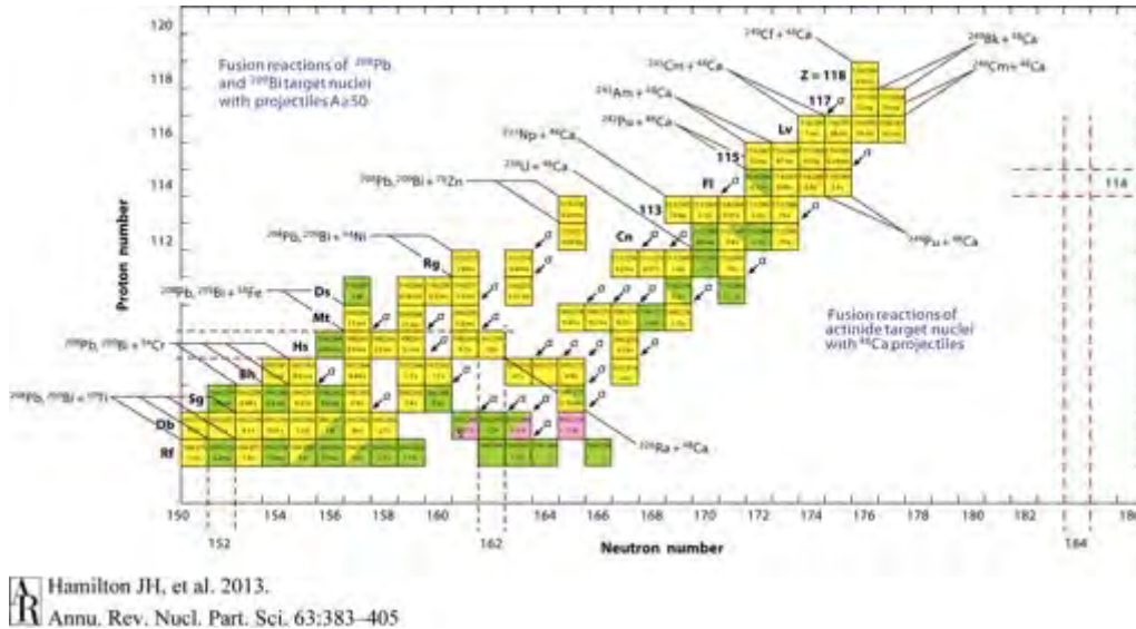
Figure 2.2: Superheavy territory, indicating some of the most recent discoveries, their production reaction, and decay chains.
