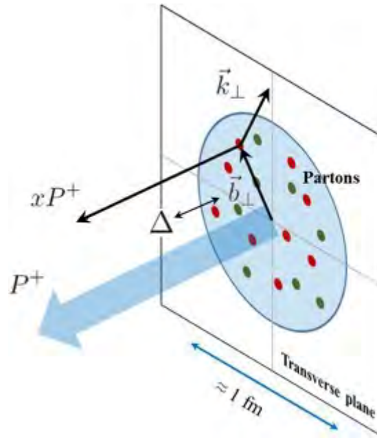
Figure 3.2: Partonic picture of hadrons. Quarks and gluons are characterized by their momentum and/or position relative to their parent hadron
