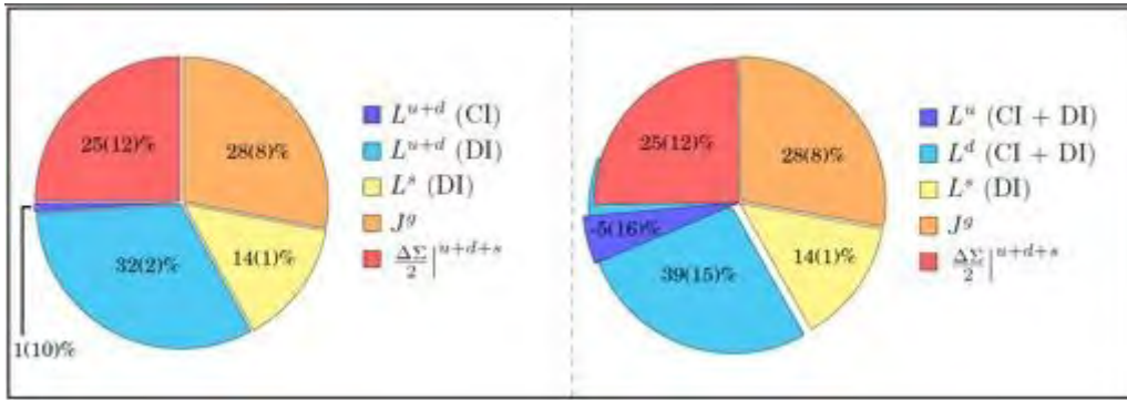
Figure 3.4: Pie charts for the quark and gluon spin and OAM fractions. The left panel shows the quark contributions separately for connected (CI) and disconnected insertions (DI), and the right panel shows the quark contributions for each flavor with CI and DI contributions summed together.
