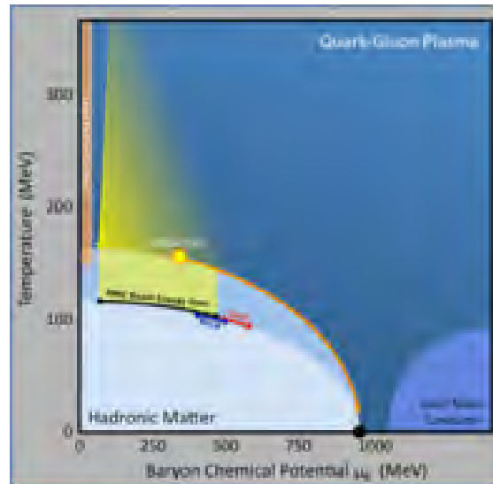
Figure 4.1: Anticipated phase structure of hadronic matter.
