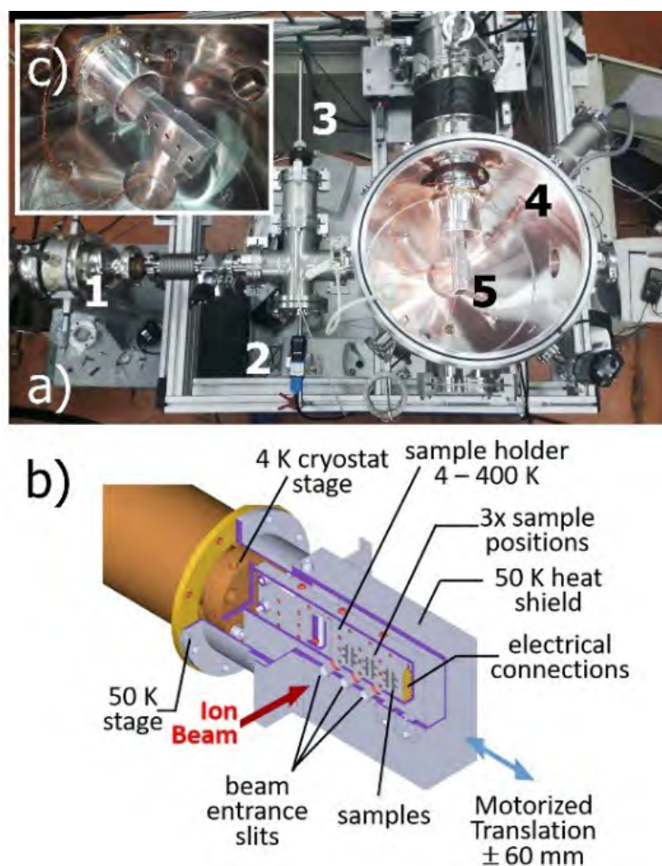
Figure 13.33: The IR2 material irradiation setup. Panel (a) shows: Ta slits (1), CCD camera (2), Faraday cup (3), vacuum chamber (4) and target holder position (5). Panel (b) depicts the individual parts of the target holder that is shown in panel (c).
