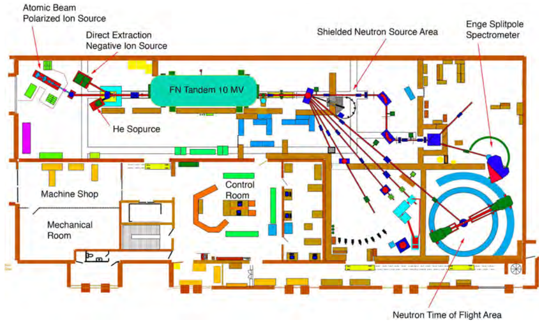
Figure 14.33: Layout of tandem laboratory.
