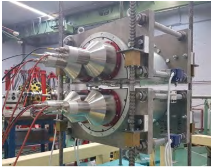
Figure 13.30: The NEOPTOLEMOS Summing Spectrometer.
